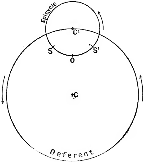
Fig. 29. The Epicycle.
